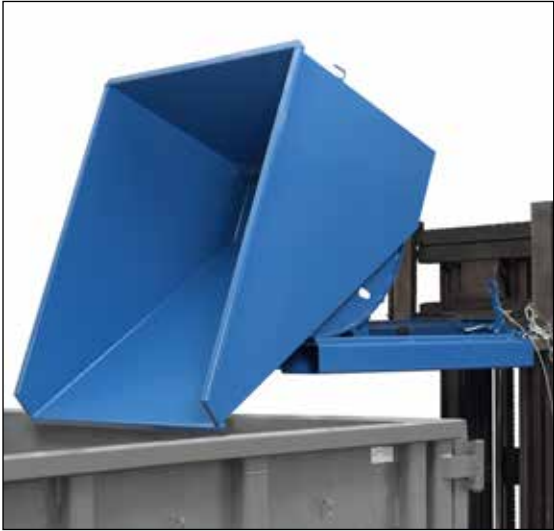
Self-tilting box as waste bin with fork-lift.
